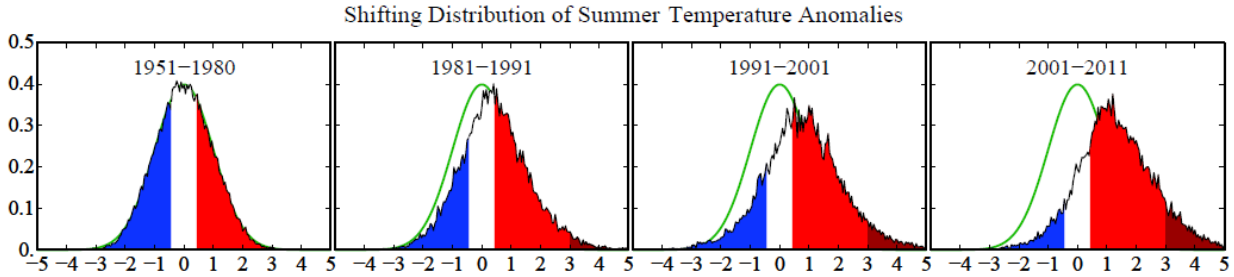
Figure 3. Frequency of occurrence (vertical axis) of local June-July-August temperature anomalies (relative to 1951-1980 mean) for Northern Hemisphere land in units of local standard deviation (horizontal axis). Temperature anomalies in the period 1951-1980 match closely the normal distribution ("bell curve", shown in green), which is used to define cold (blue), typical (white) and hot (red) seasons, each with probability 33.3%. The distribution of anomalies has shifted to the right as a consequence of the global warming of the past three decades such that cool summers now cover only half of one side of a six-sided die, white covers one side, red covers four sides, and an extremely hot (red-brown) anomaly covers half of one side..
